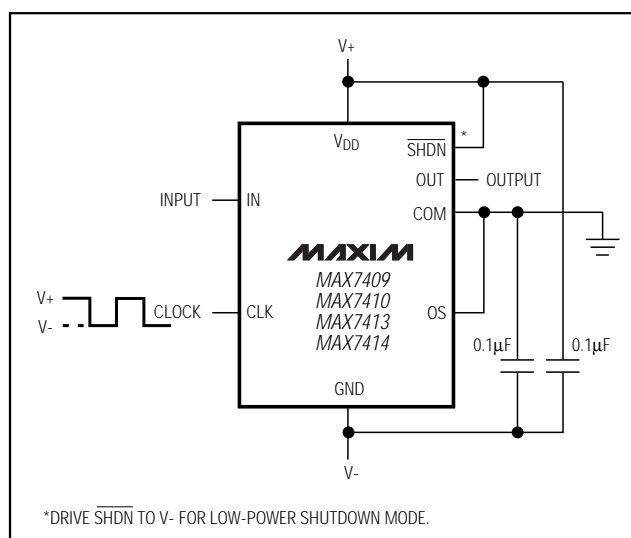
Figure 4. Dual-Supply Operation
