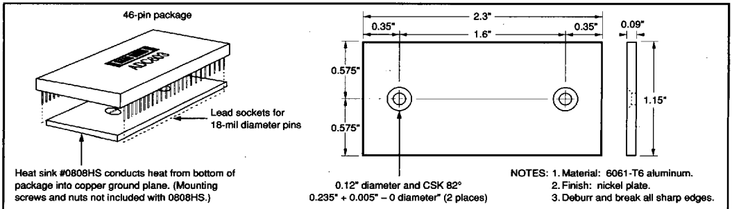
FIGURE 20. Heat Sink Transfers Heat from the DIP Package into a Copper Ground Plane.
