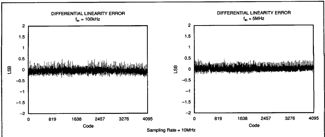
FIGURE 16. 100kHz and 5MHz Differential Linearity.
