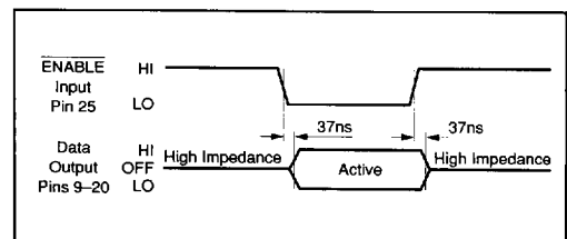
FIGURE 22. Digital Data Tri-State Output.
