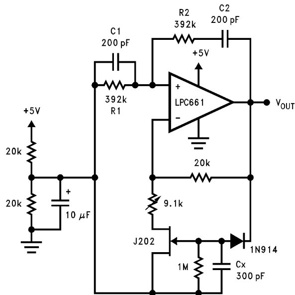
Sine-Wave Oscillator
