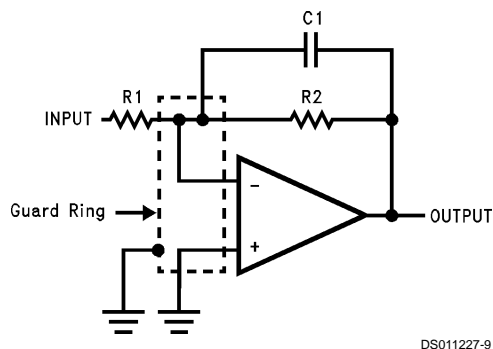
FIGURE 5. Inverting Amplifier Guard Ring Connections
