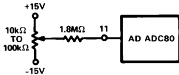
Figure 7. Offset Adjustment Circuit
