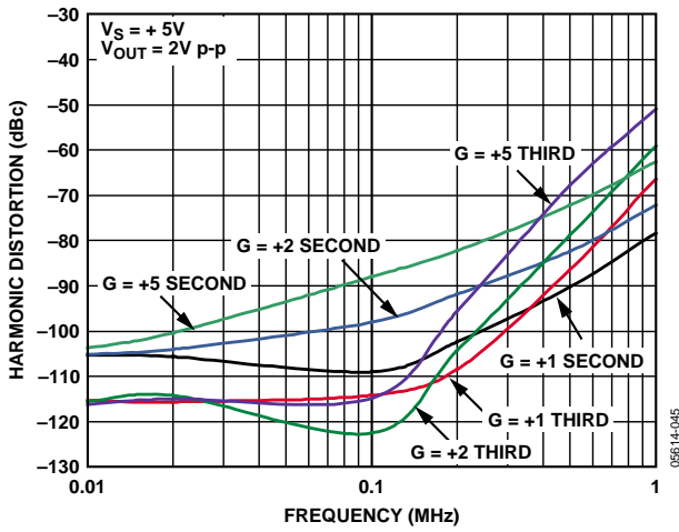
Figure 11. Harmonic Distortion vs. Frequency for Various Gains
