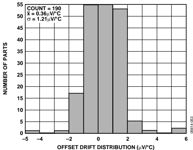
Figure 16. Input Offset Voltage Distribution
