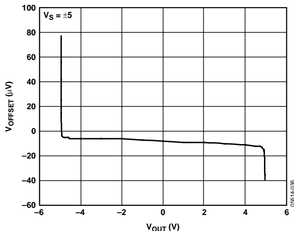
Figure 18. Input Error Voltage vs. Output Voltage
