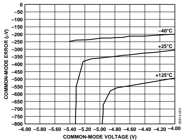
Figure 41. V_{OS} vs. -CMP vs. Common-Mode Error
