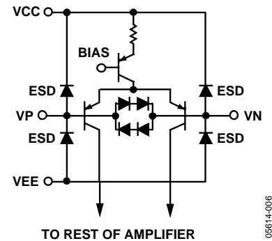
Figure 45. Input Stage and Protection Diodes
