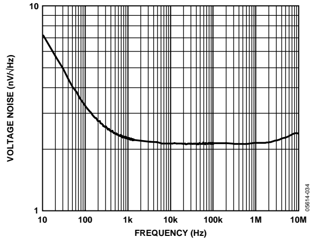
Figure 14. Voltage Noise vs. Frequency
