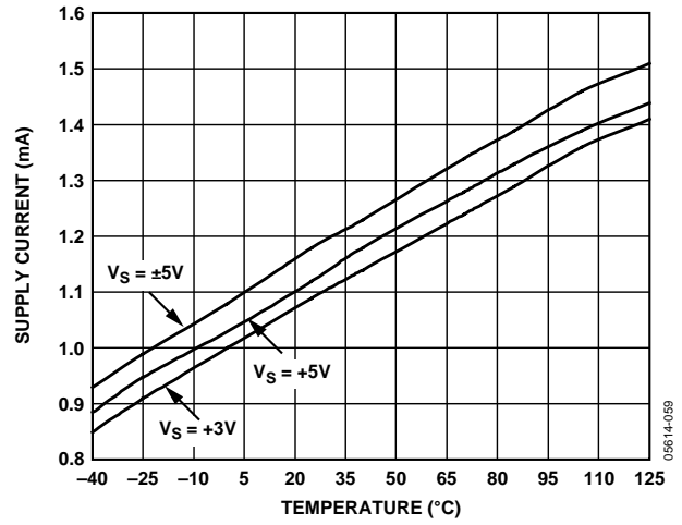
Figure 36. Supply Current vs. Temperature for Various Supplies
