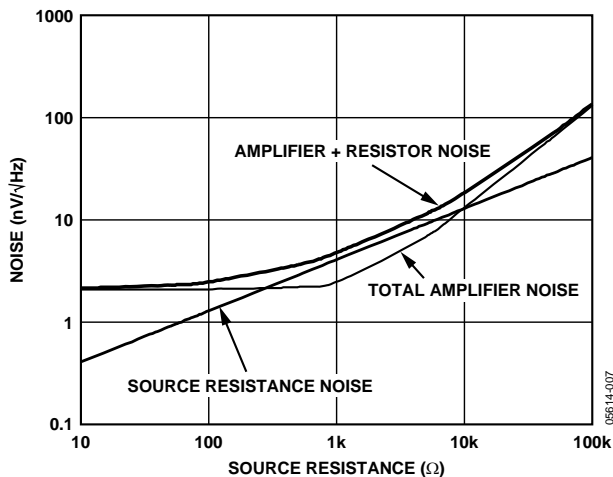
Figure 39. RTI Noise vs. Source Resistance
