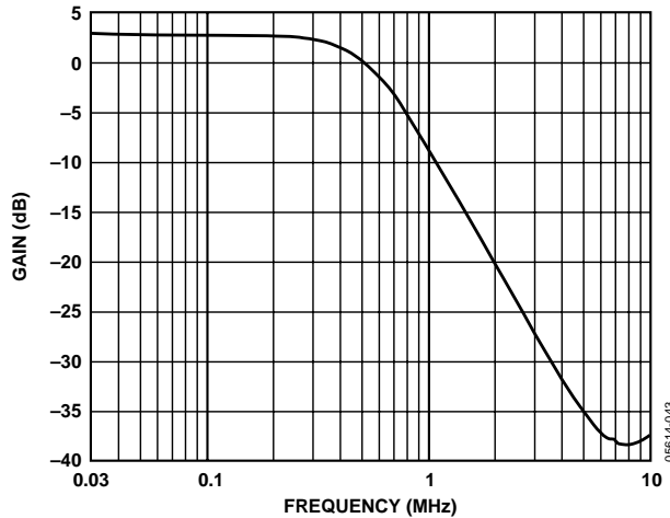
Figure 49. Filter Frequency Response
