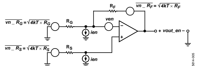
Figure 38. Noise Sources in Typical Connection
