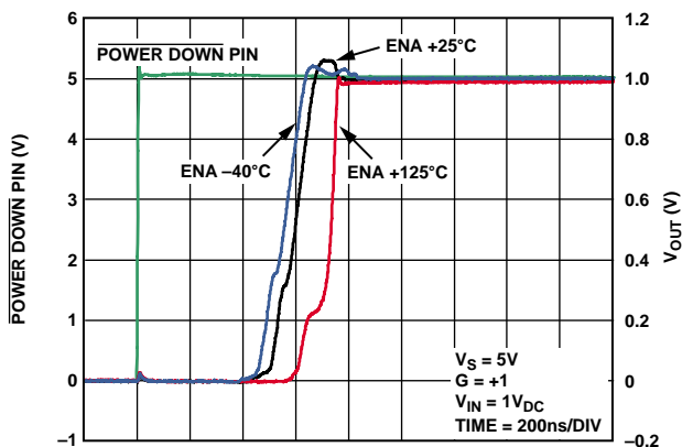
Figure 28. Power-Up Time vs. Temperature
