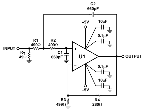
Figure 48. Two-Pole 500 kHz Reconstruction Filter Schematic
