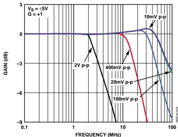
Figure 9. Frequency Response for Various V_{OUT}
