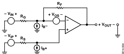
Figure 37. Typical Connection Diagram and DC Error Sources
