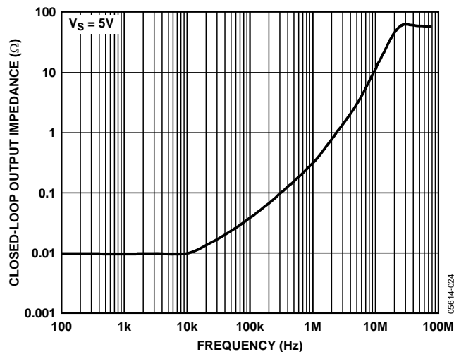
Figure 33. Output Impedance vs. Frequency
