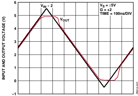
Figure 23. Output Overdrive Recovery
