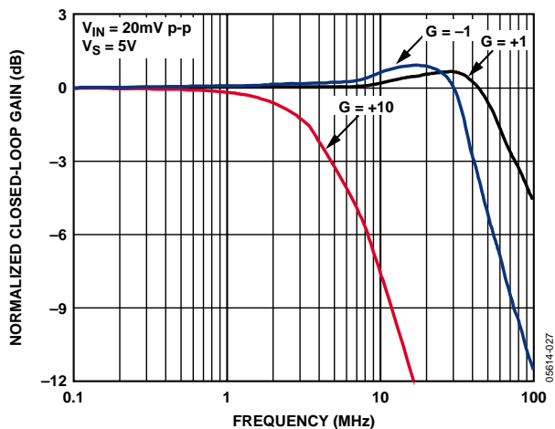
Figure 6. Small Signal Frequency Response vs. Gain
