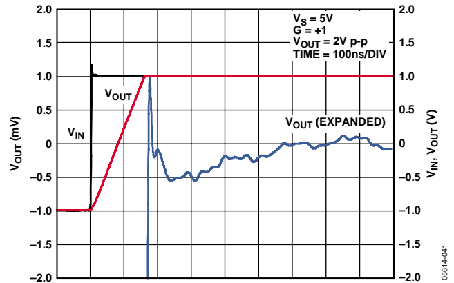
Figure 27. Settling Time
