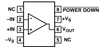
Figure 1. 8-Lead SOIC (R)
