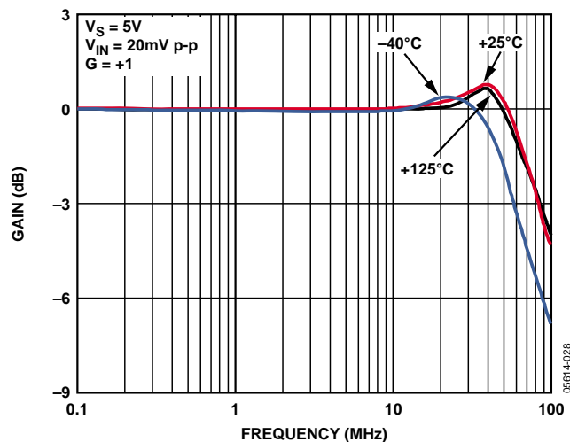
Figure 7. Small Signal Frequency Response vs. Temperature
