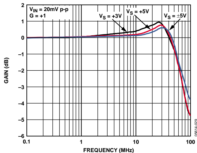
Figure 8. Small Signal Frequency Response vs. Supply Voltage
