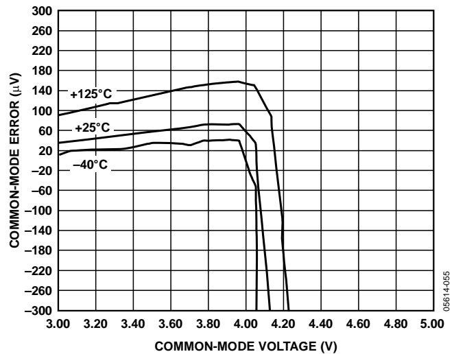
Figure 40. V_{OS} vs. +CMP vs. Common-Mode Error
