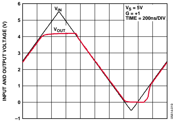
Figure 22. Input Overdrive Recovery
