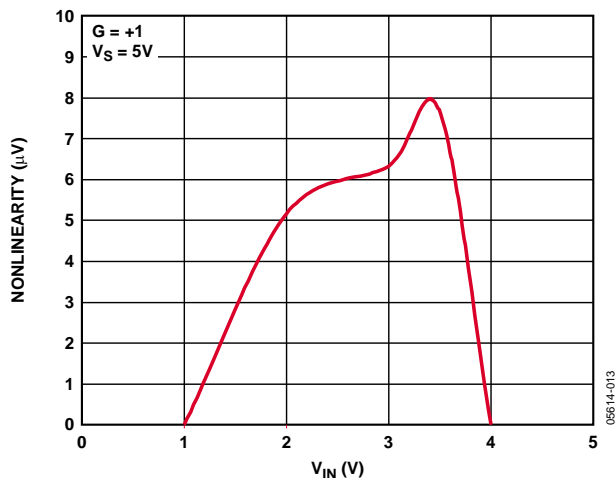
Figure 17. Nonlinearity vs. V_{IN}
