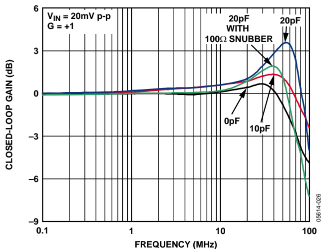
Figure 5. Small Signal Frequency Response vs. Capacitive Load
