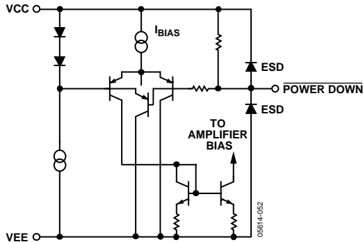
Figure 46. Power-Down Circuit
