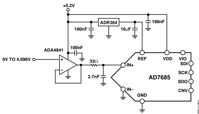
Figure 47. ADC Driver Schematic
