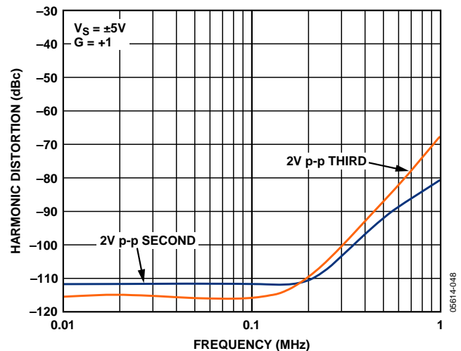
Figure 2. Harmonic Distortion
