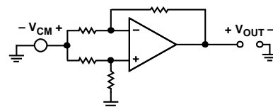
Figure 42. Common-Range Subtractor
