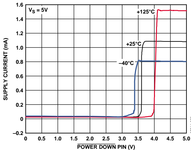
Figure 30. Supply Current vs. POWER DOWN Pin Voltage
