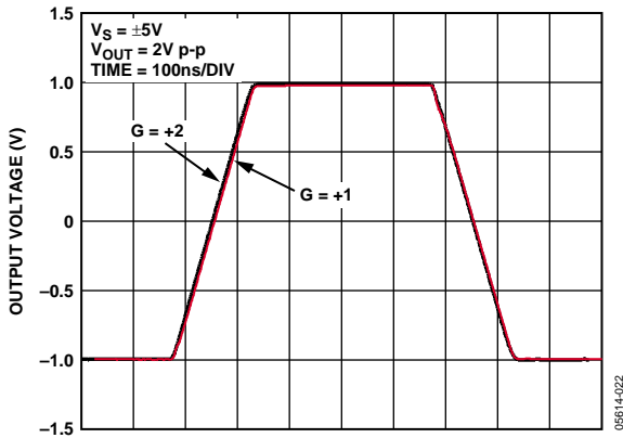
Figure 24. Large Signal Transient Response for Various Gains
