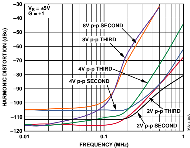
Figure 12. Harmonic Distortion vs. Frequency for Various Output Voltages
