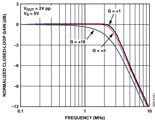
Figure 4. Large Signal Frequency Response vs. Gain
