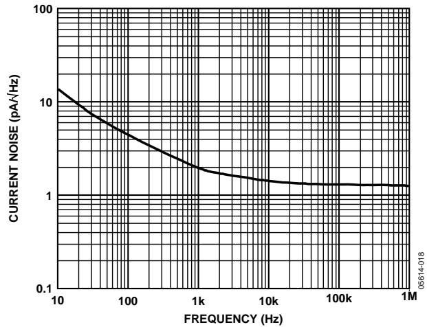
Figure 15. Current Noise vs. Frequency
