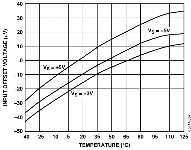
Figure 34. Input Offset Voltage vs. Temperature for Various Supplies
