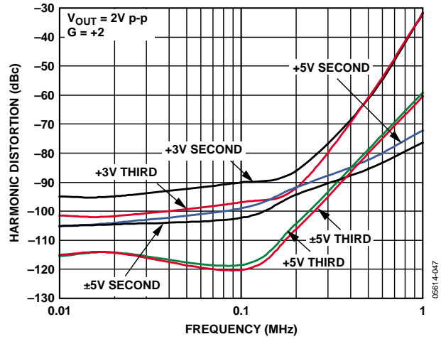
Figure 13. Harmonic Distortion vs. Frequency for Various Supplies
