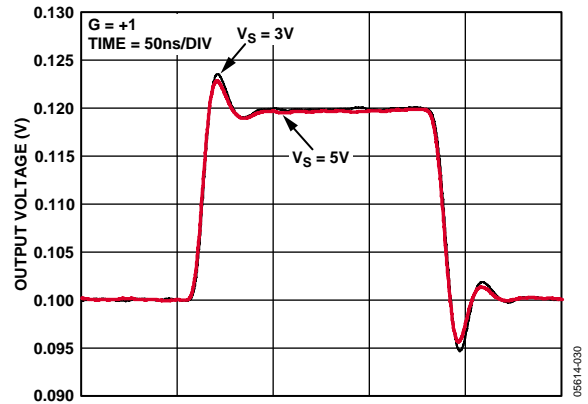
Figure 25. Small Signal Transient Response for Various Supplies
