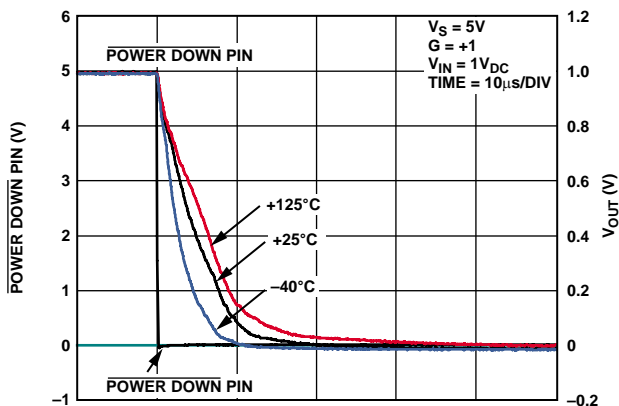
Figure 29. Power-Down Time vs. Temperature
