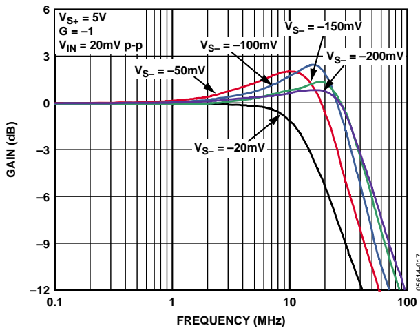
Figure 43. Small Signal Frequency Response vs. Negative Supply Bias
