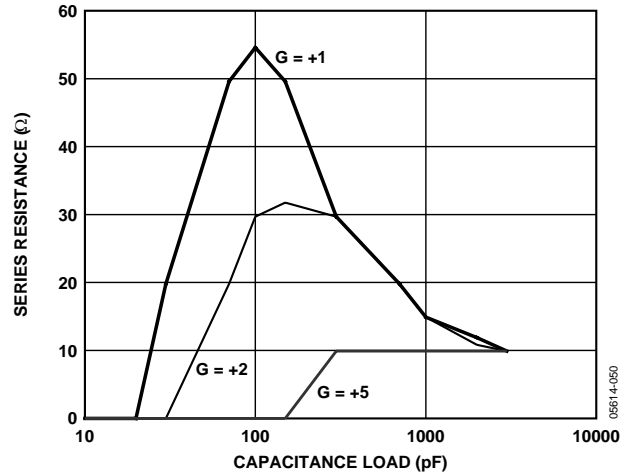
Figure 44. Series Resistance vs. Capacitive Load
