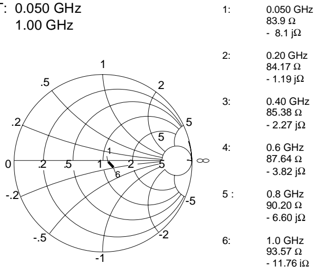
Figure 9: Output Impedance
