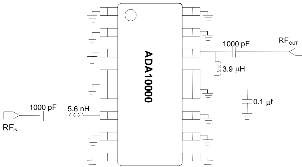
Figure 3: Test Circuit
