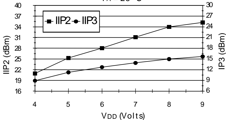
Figure 6: IIP2, IIP3 vs. VDD
