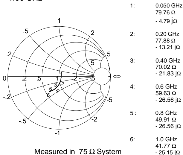
Figure 9: Output Impedance
