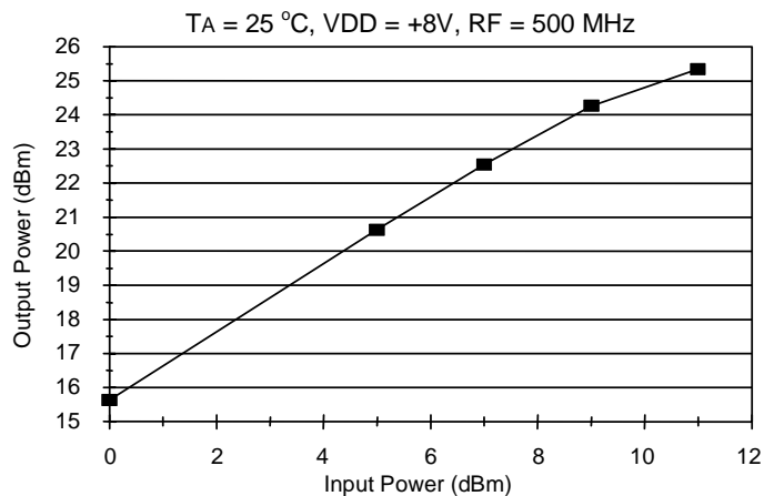
Figure 7: Output Power vs. Input Power
