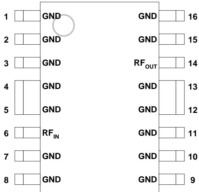
Figure 2: Pin Out
