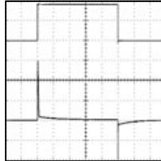
LOAD TRANSIENT ( V_{OUT} = 10V , C_{OUT} = 0 , 0 TO 20mA)
