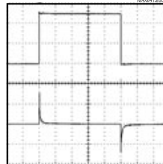
LOAD TRANSIENT ( V_{OUT} = 2.5V , C_{OUT} = 0 , 0 TO -2mA)
