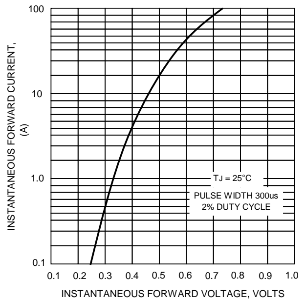
FIG.4-TYPICAL FORWARD CHARACTERISTICS
