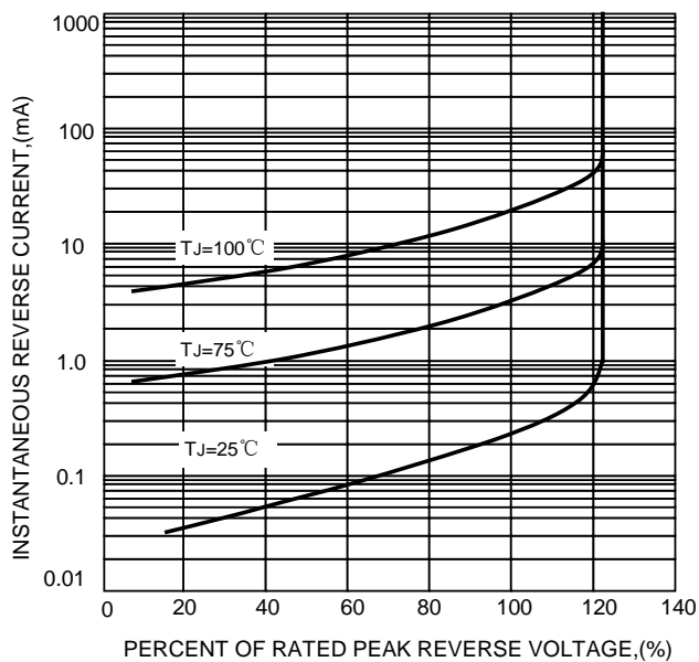
FIG.3-TYPICAL REVER CHARACTERISTICS
