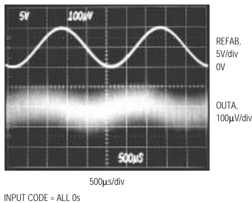
MAX536 REFERENCE FEEDTHROUGH AT 400Hz
