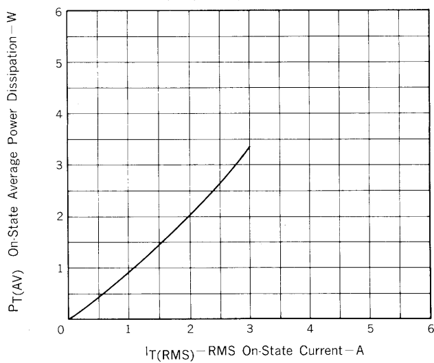
Fig. 11 P_{T(AV)} - I_{T(RMS)} CHARACTERISTIC
