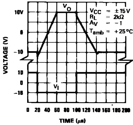
INVERTING LARGE SIGNAL PULSE RESPONSE (LM148)
