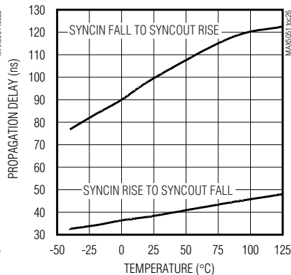
SYNCIN TO SYNCOUT PROPAGATION DELAY vs. TEMPERATURE
