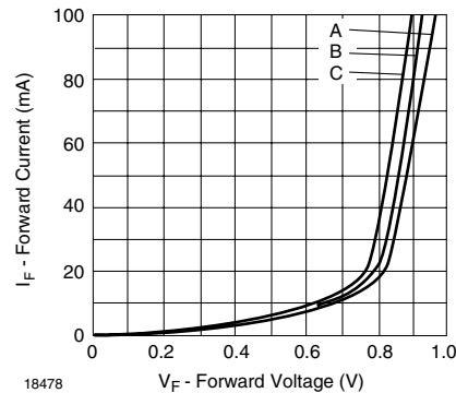
Figure 2. Typical Forward Conduction Curve
