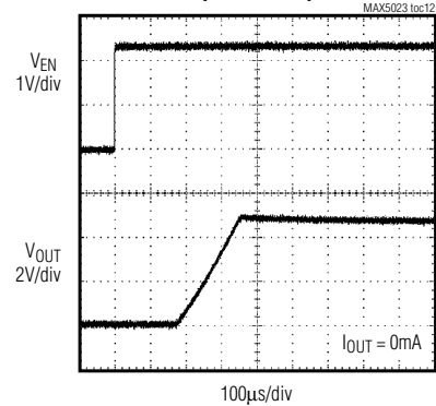
ENABLE STARTUP RESPONSE ( V_{\text{IN}} = +14\text{V} )
