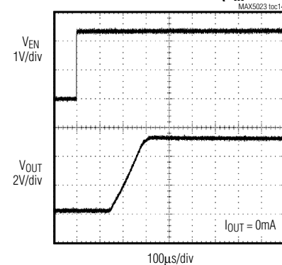
ENABLE STARTUP RESPONSE ( V_{\text{IN}} = +65\text{V} )
