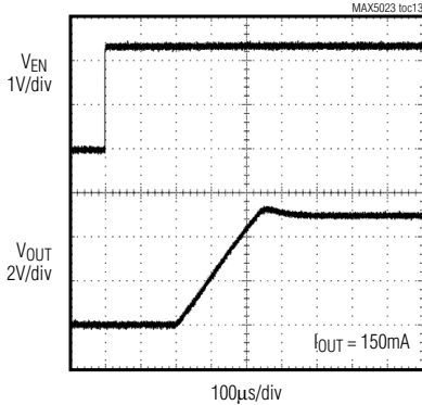
ENABLE STARTUP RESPONSE ( V_{\text{IN}} = +14\text{V} )
