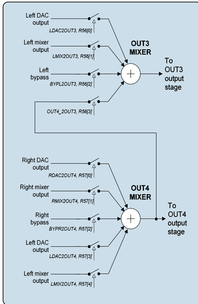
Figure 33 OUT3 and OUT4 Mixers
