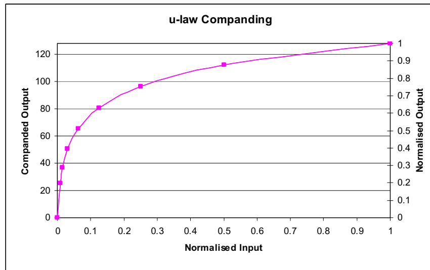
Figure 44 u-Law Comanding
