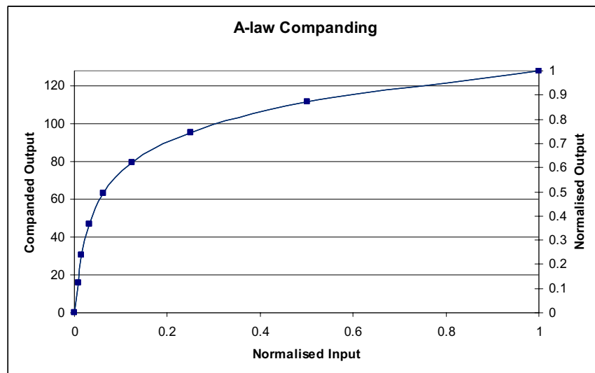
Figure 45 A-Law Comanding
