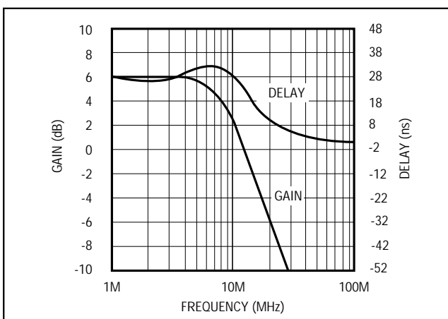
Figure 10b. Gain and Delay vs. Frequency
