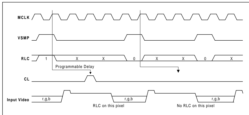
Figure 17 Relationship of RLC pin, MCLK and VSMP to Internal Clamp Pulse, CL
