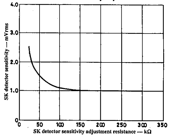
SK detector sensitivity adjustment
