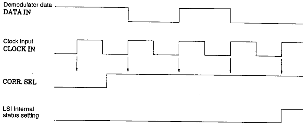
Figure 5. CORR.SEL read timing during sync detection
