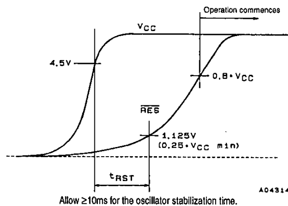
Figure 2. Reset time
