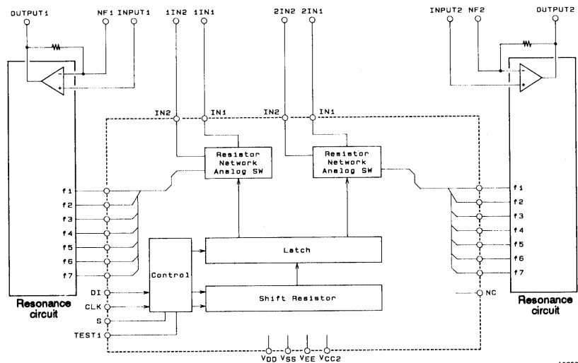
Figure 1 Equivalent Circuit Block Diagram
