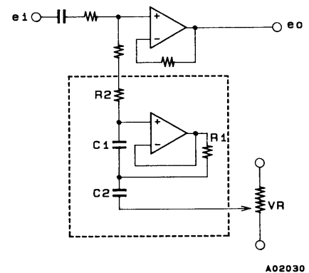
Figure 2 Resonance Circuit
