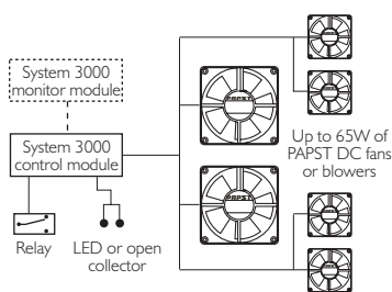
Alarm outputs
