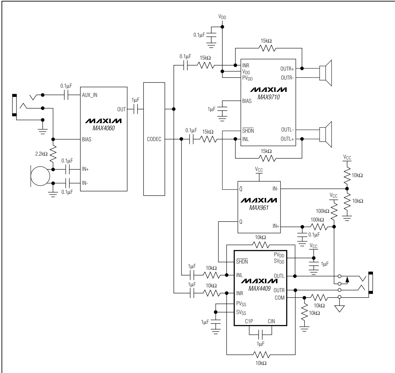
System Diagram
