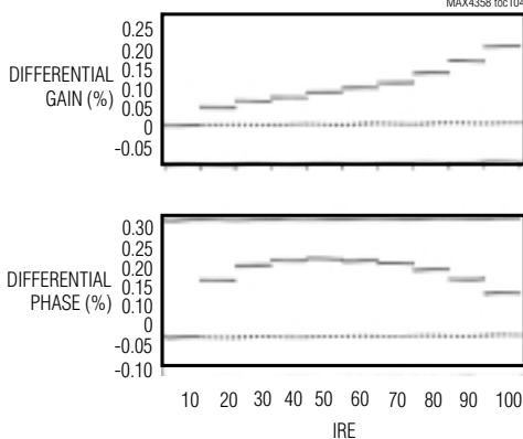
DIFFERENTIAL GAIN AND PHASE (RL = 150Ω)
