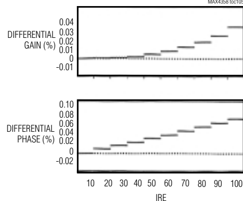
DIFFERENTIAL GAIN AND PHASE (RL = 1kΩ)
