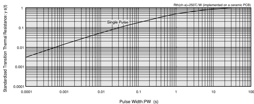
STANDARDIZED TRANSITION THERMAL RESISTANCE vs. PULSE WIDTH
