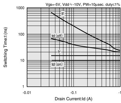
SWITCHING TIME vs. DRAIN CURRENT
