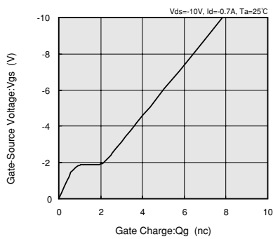
GATE-SOURCE VOLTAGE vs. GATE CHARGE
