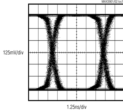
OUTPUT EYE DIAGRAM (2µAp-p ELECTRICAL INPUT AT T_J = -40^\circ C )
