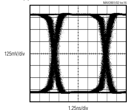
OUTPUT EYE DIAGRAM (2µAp-p ELECTRICAL INPUT AT T_J = +140^\circ C )
