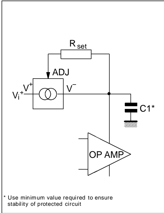
Figure 9 : In-line Current Limiter
