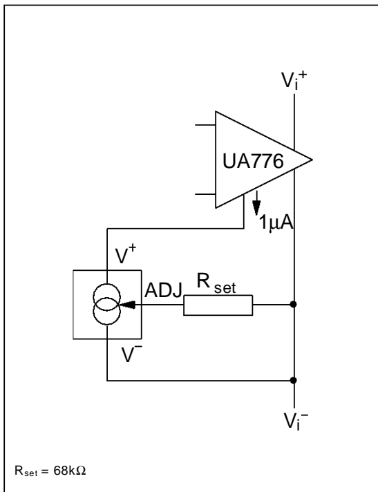
Figure 7 : Micropower Bias
