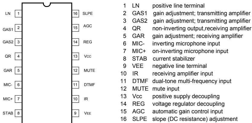
Fig.2 PIN CONFIGURATIONS
