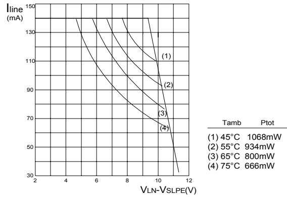
Fig.6 UTC TEA1062N/TEA1062AN safe operating area
