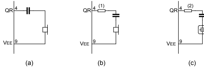
Fig.11 Alternative receiver arrangement
