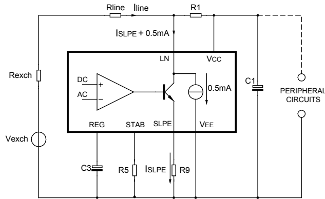
Fig.8 Supply arrangement
