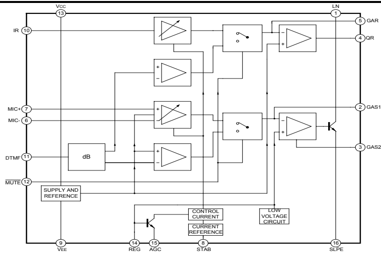
Fig.1 Block Diagram
