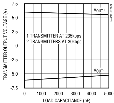
MAX3243 TRANSMITTER OUTPUT VOLTAGE vs. LOAD CAPACITANCE
