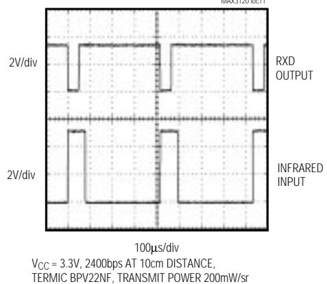
RXD OUTPUT vs. INFRARED INPUT
