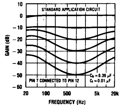
FIGURE 7. Loudness Compensated Volume Characteristic
