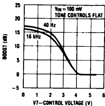
Loudness Control Characteristic
