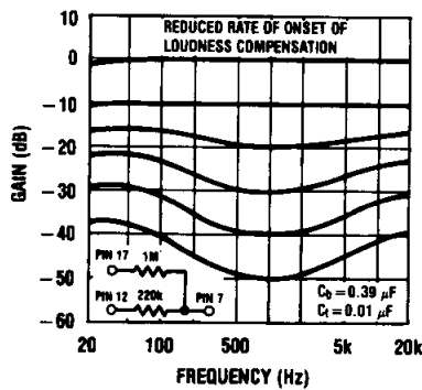
FIGURE 10. Loudness Compensated Volume Characteristic
