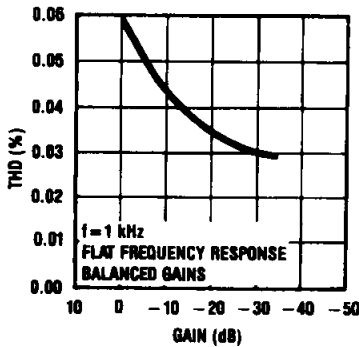
THD vs Gain
