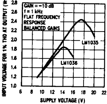
Input Signal Handling vs Supply Voltage
