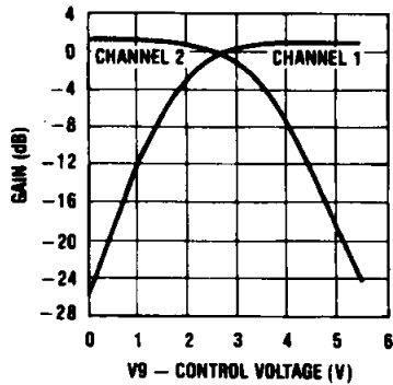
Balance Control Characteristic
