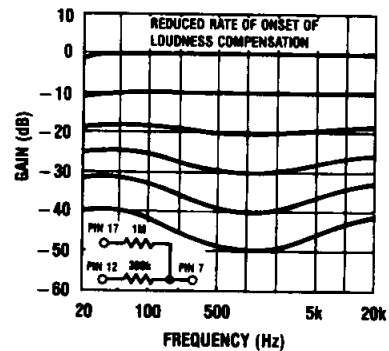
FIGURE 11. Loudness Compensated Volume Characteristic
