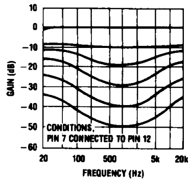
Loudness Compensated Volume Characteristic
