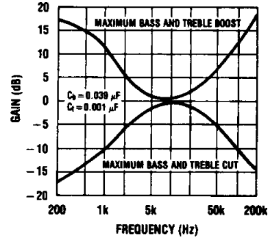
FIGURE 15. Tone Characteristic (Gain vs Frequency)
