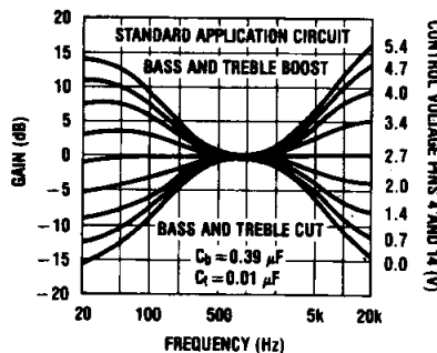
FIGURE 1. Tone Characteristic (Gain vs Frequency)
