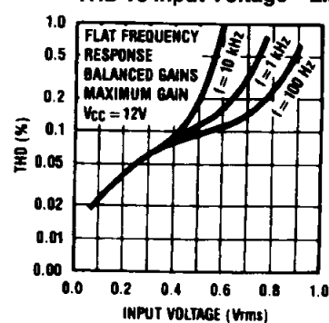
THD vs Input Voltage—LM1036
