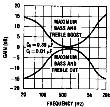
Tone Characteristic (Gain vs Frequency)
