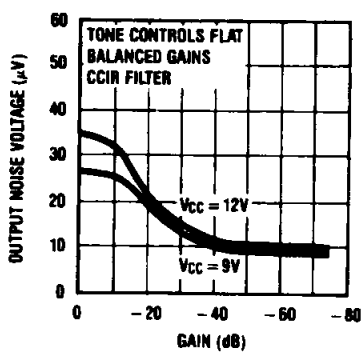
Output Noise Voltage vs Gain—LM1036
