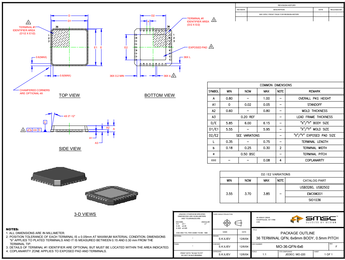
Figure 9.1 36 Pin QFN Package
