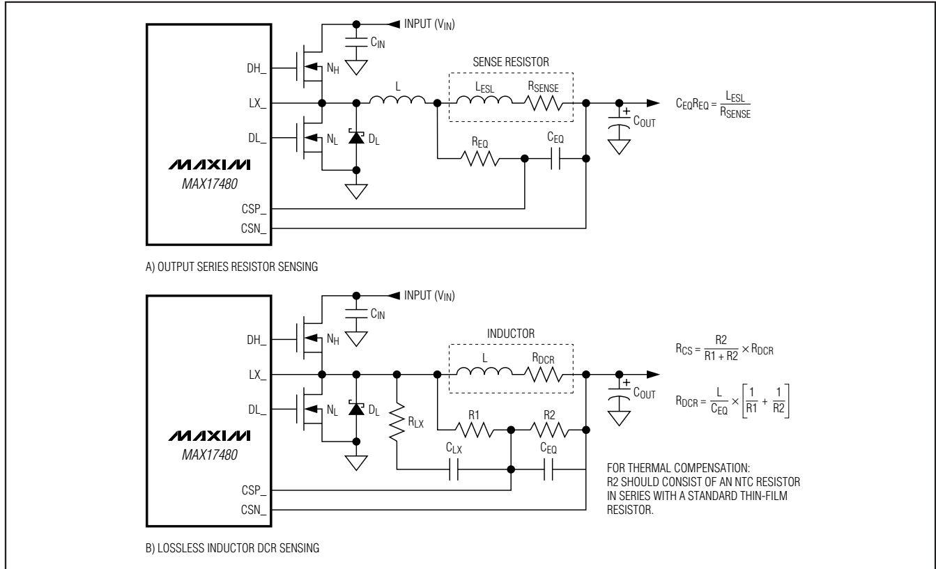
Figure 7. Current-Sense Configurations
