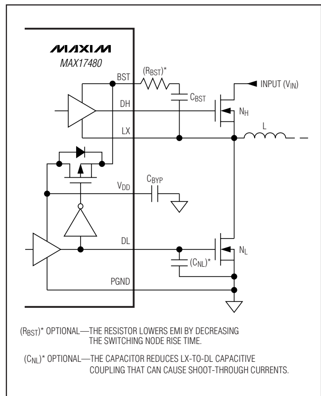
Figure 11. Gate-Drive Circuit
