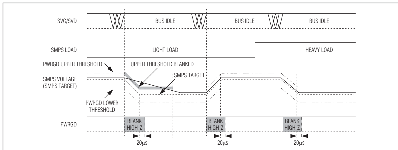
Figure 6. VID Transition Timing
