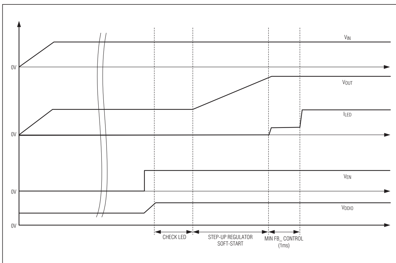
Figure 3. Startup Sequence
