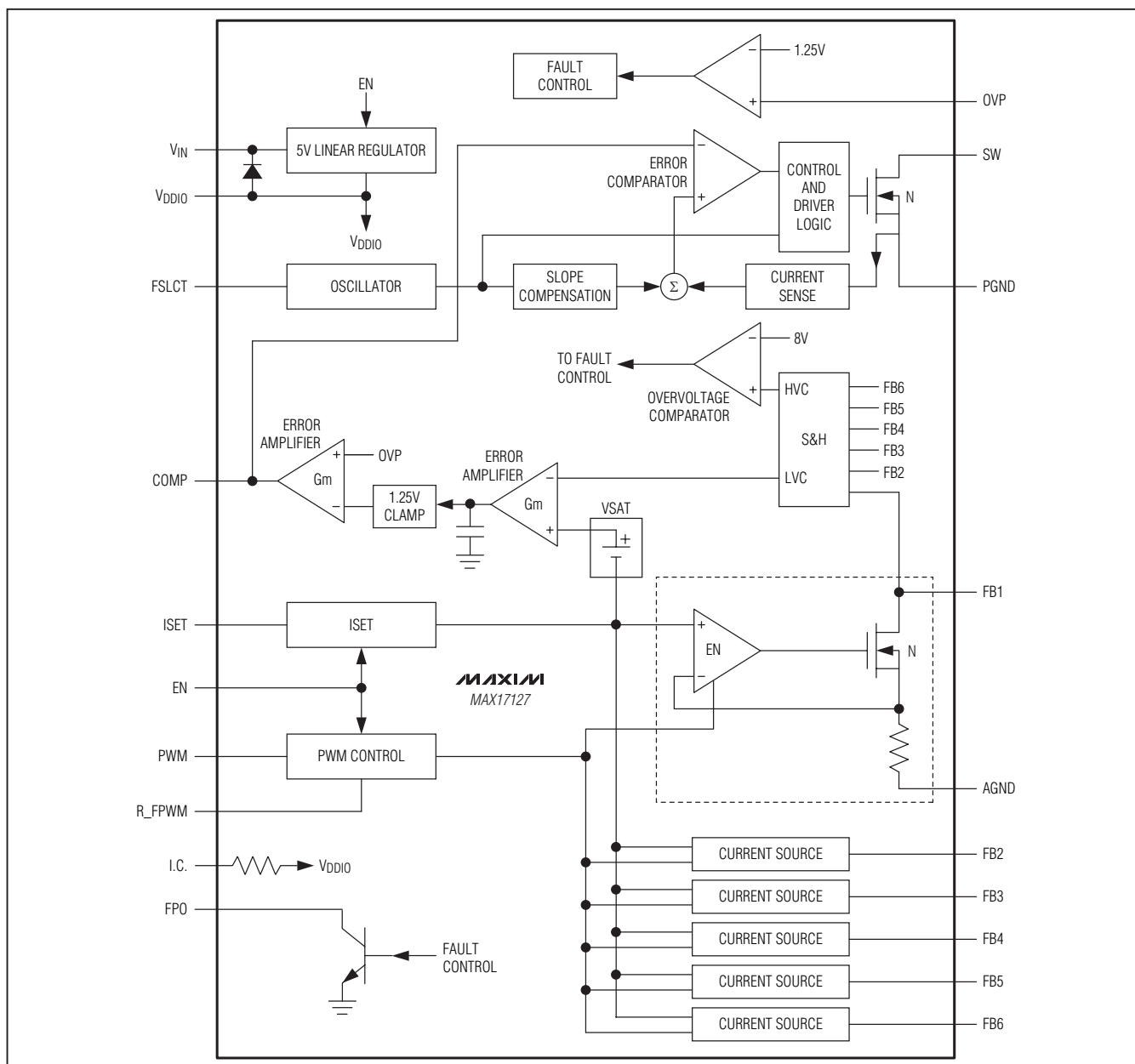
Figure 2. Functional Diagram
