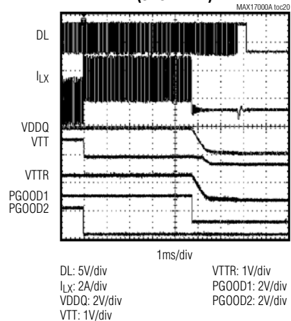
VTT OVERLOAD FAULT WAVEFORMS (5ms TIMER)
