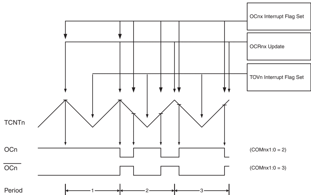
Figure 20-7. Phase Correct PWM Mode, Timing Diagram
