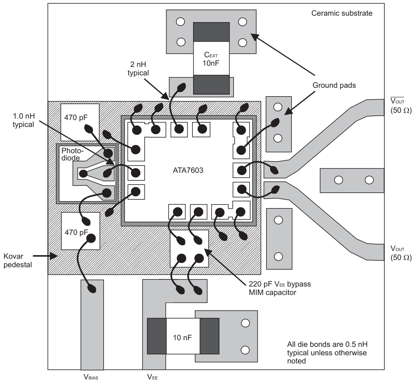
Figure 15: Bonding Diagram
