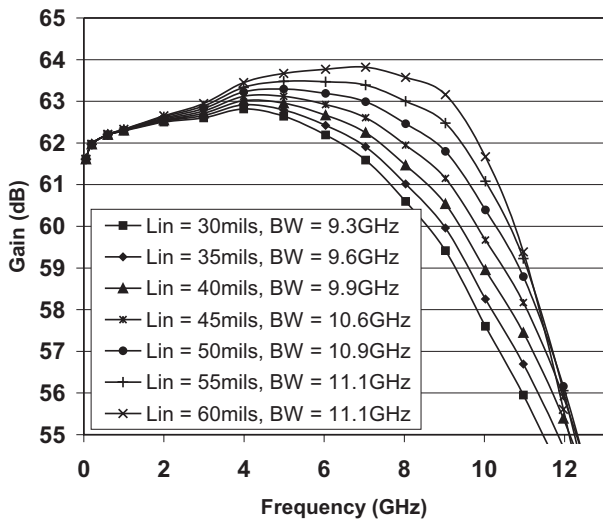
Figure 5: Bandwidth vs. Input Inductance
