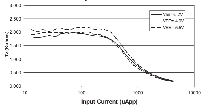
Figure 6: Differential Transimpedance vs. Input Current
