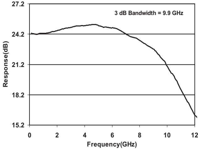
Figure 3: Typical Small Signal Frequency Response
