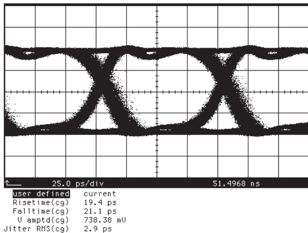
Figure 13: Eye Diagram with an Optical Input Power of +4 dBm
