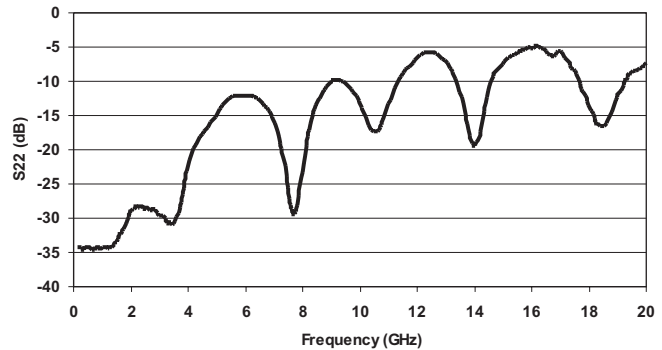
Figure 14: S22 from Evaluation Test Fixture
