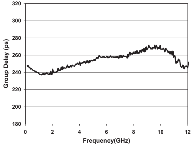
Figure 4: Typical Small Signal Group Delay
