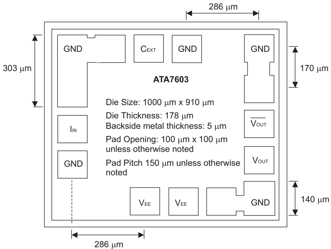
Figure 2: Die Size and Layout
