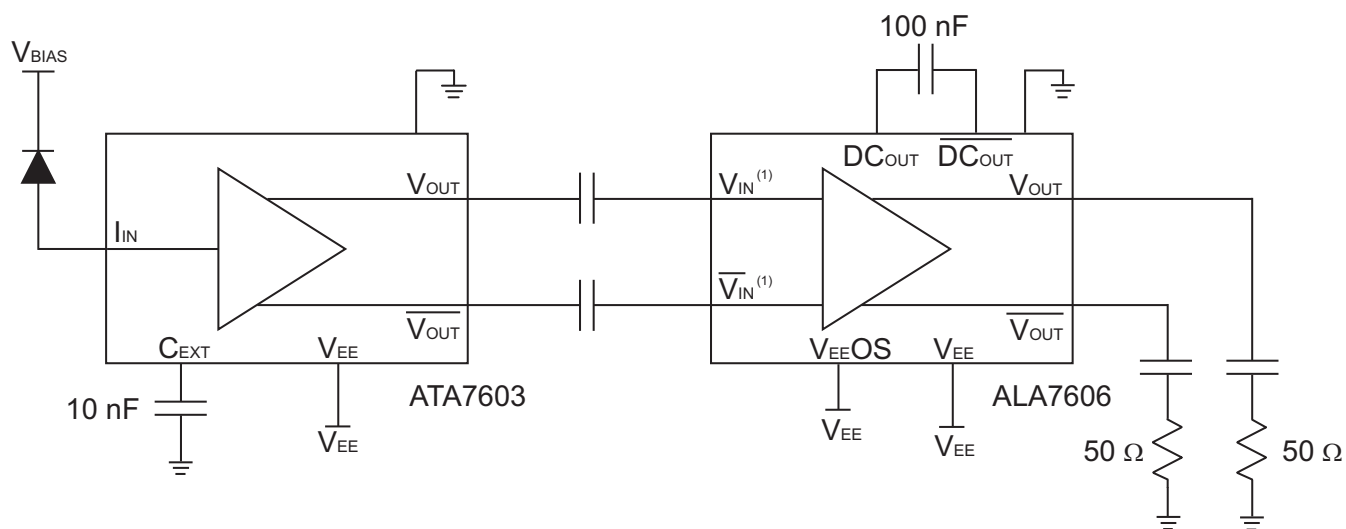
Figure 17: ATA7603 AC Coupled to the ALA7606
