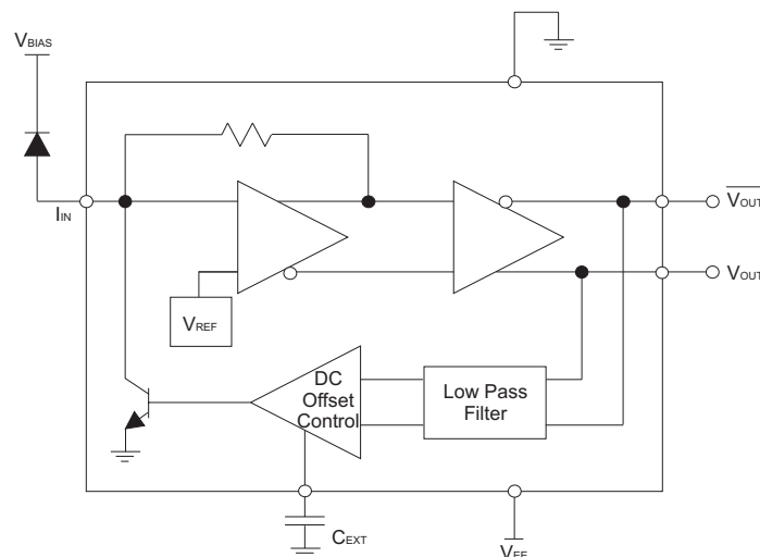
Figure 1: Circuit Block Diagram
