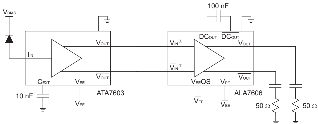
Figure 16: ATA7603 DC Coupled to the ALA7606
