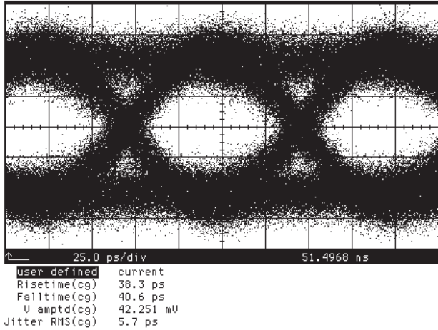
Figure 9: Eye Diagram with an Optical Input Power of -18 dBm
