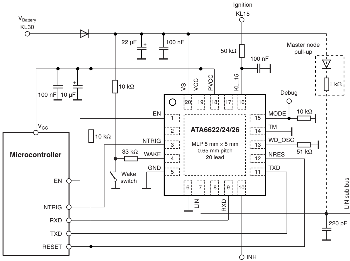
Figure 8-2. Application Circuit
