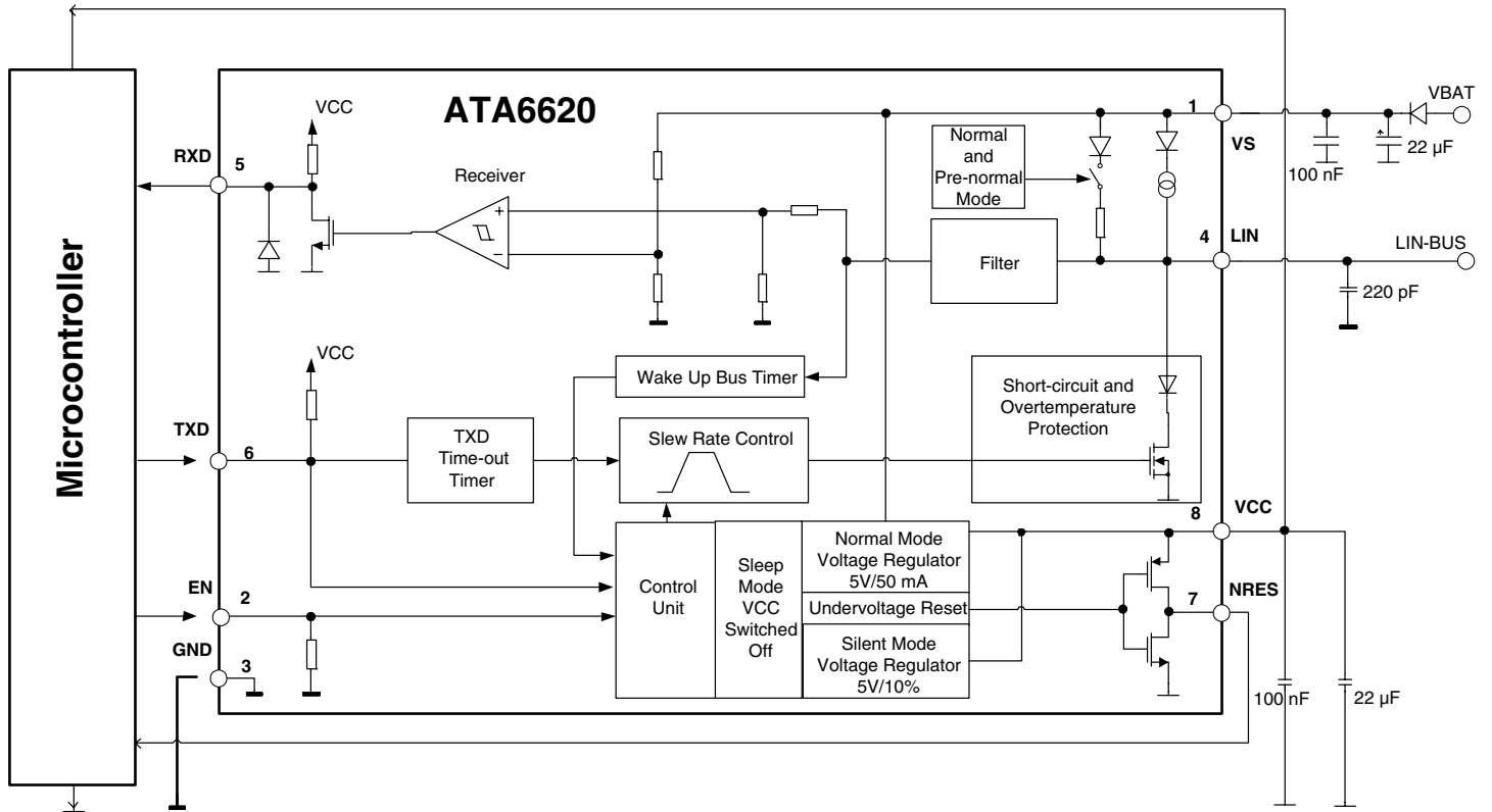
Figure 8-2. Application Circuit
