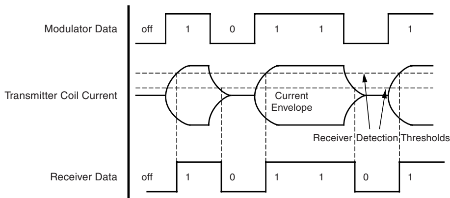
Figure 3-13. Example for OOK-data Modulation with ATA5279
