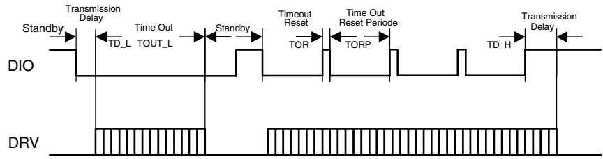
Figure 8. Time Out and Time Out Reset Protocol
