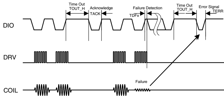
Figure 9. Transmission Acknowledge and Error Signal
