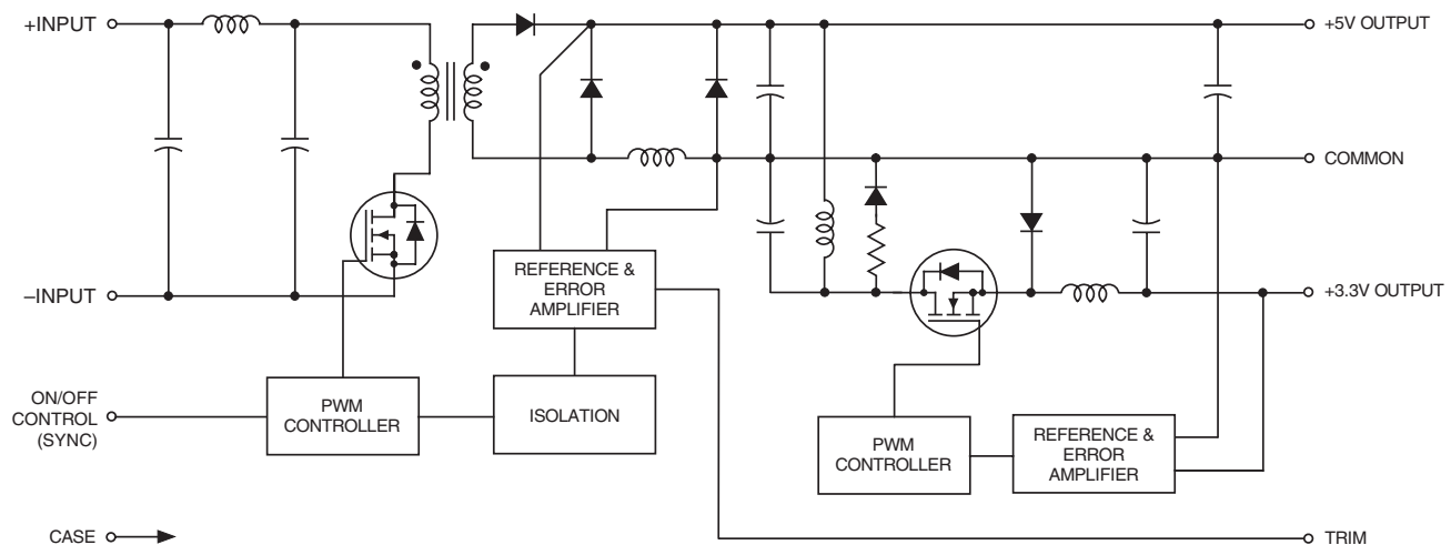
Figure 1. Simplified Schematic
