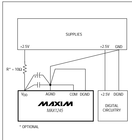
Figure 16. Power-Supply Grounding Connection
