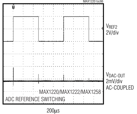
ADC REFERENCE FEEDTHROUGH RLOAD = 10kΩ, CLOAD = 100pF
