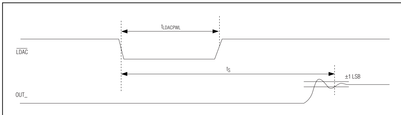
Figure 14. LDAC Functionality
