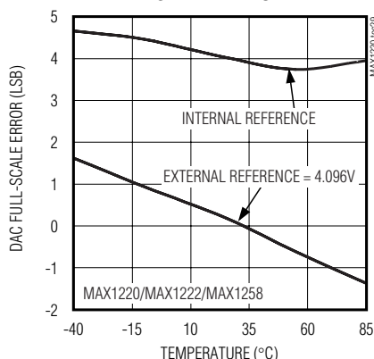
DAC FULL-SCALE ERROR vs. TEMPERATURE
