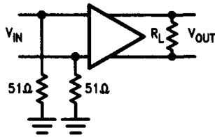
Test Circuit 1
