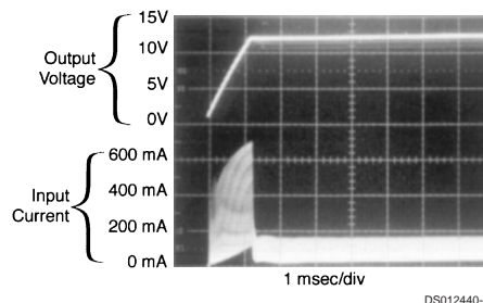
FIGURE 26. Output Voltage, Input Current, at Start-Up, WITHOUT Soft-start
