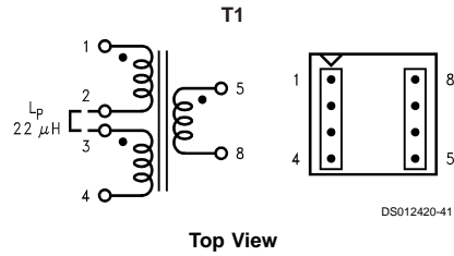
Top View FIGURE 25. Renco RL-5530
