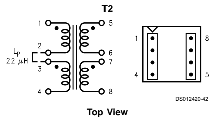
Top View FIGURE 26. Renco RL-5531
