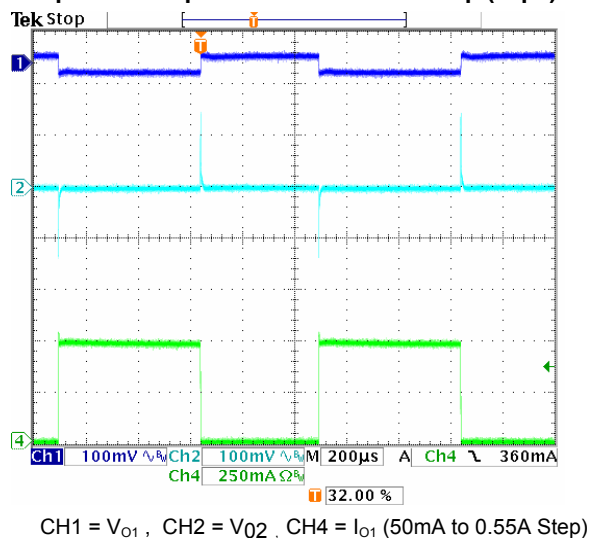
Step Load Response With Tantalum Cap (10µF)
