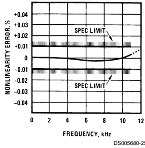
Nonlinearity Error as Precision V-to-F Converter (Figure 4)
