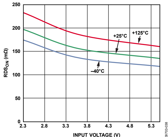
Figure 33. PMOS R_{DS(ON)} vs. V_{INx}
