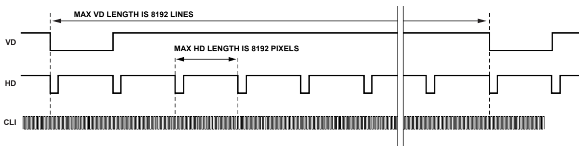
Figure 15. Maximum VD/HD Dimensions
