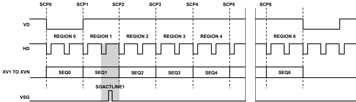
Figure 49. Complete Field is Divided into Regions
