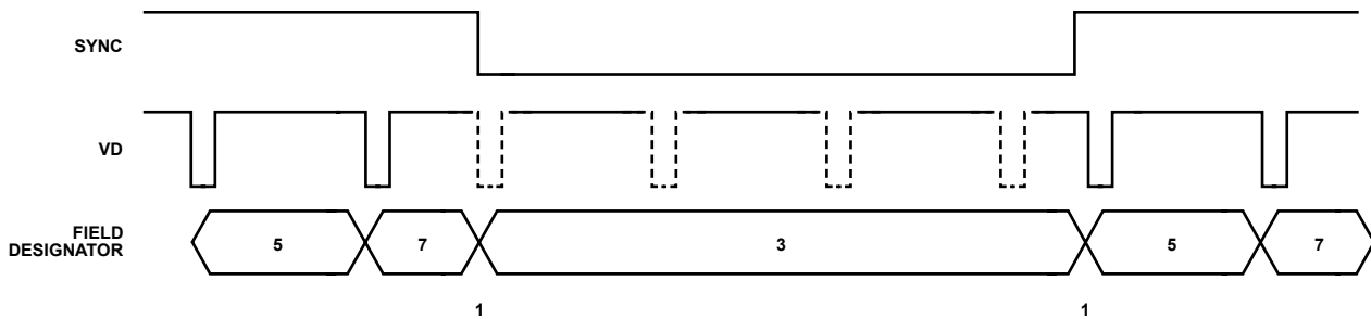
Figure 83. Special SYNC Mode Effect on Field Designator
