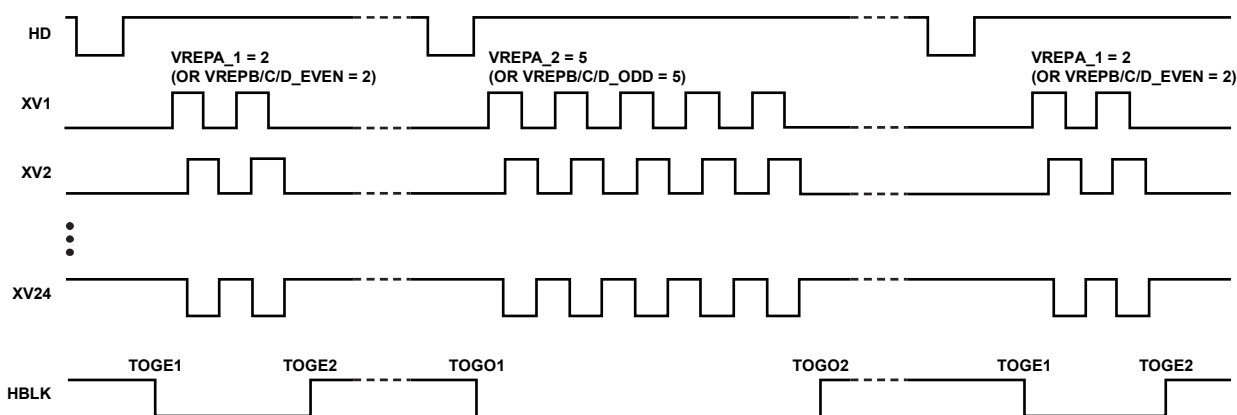
Figure 43. Odd/Even Line Alternation of V-Pattern Group Repetitions and HBLK Toggle Positions
