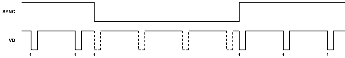
Figure 81. Enhanced SYNC Mode 3
